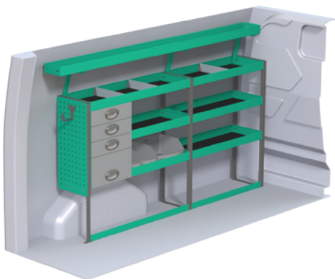
Package number F40704 W x D x H 1878x300x1000/1265 mm • Weight app. 61 kg
