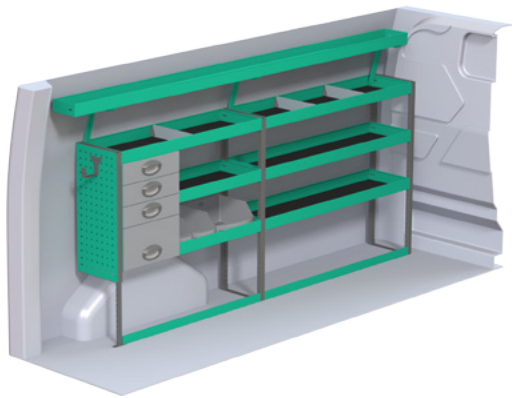
Package number F40724 W x D x H 2270x300x1000/1265 mm • Weight app. 72 kg
