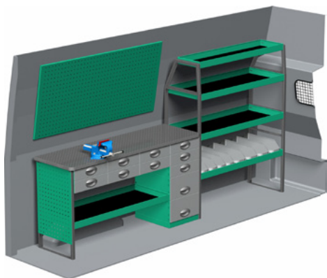
Package number F47086 W x D x H 2841 x 470 x 1510 mm • Weight app. 139 kg
