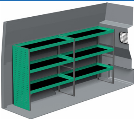
Package number F47060 W x D x H 2449 x 470 x 1220 mm • Weight app. 59 kg
