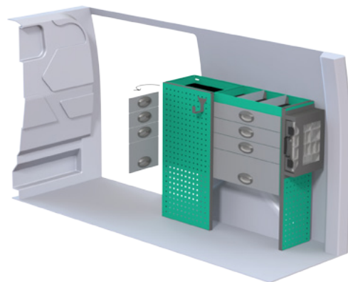
Package number F40705 W x D x H 1197x300x1000 mm • Weight app. 57 kg
