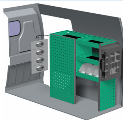
Package number F40063 W x D x H 980 x 300 x 890 mm • Weight app. 36 kg
