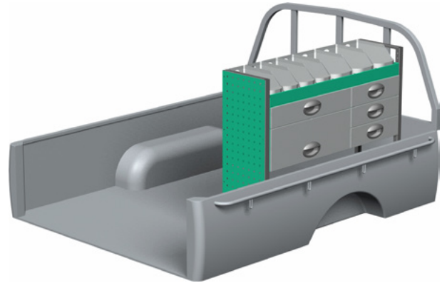
Package number F40103 W x D x H 1062 x 300 x 890 mm • Weight app. 34 kg
