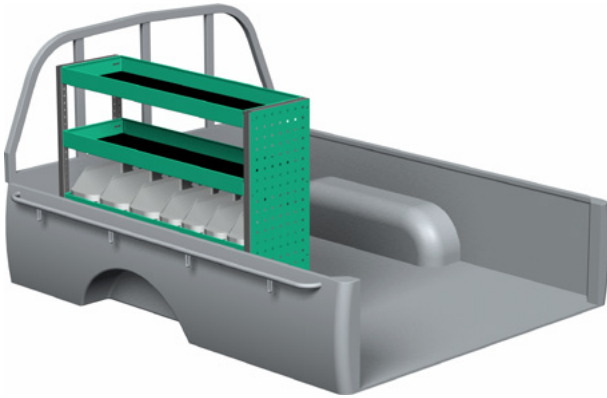
Package number F40100 W x D x H 1062 x 300 x 890 mm • Weight app. 22 kg
