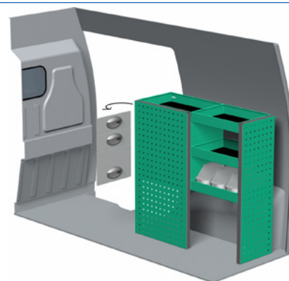
Package number F40081 W x D x H 895 x 300 x 890 mm • Weight app. 31 kg
