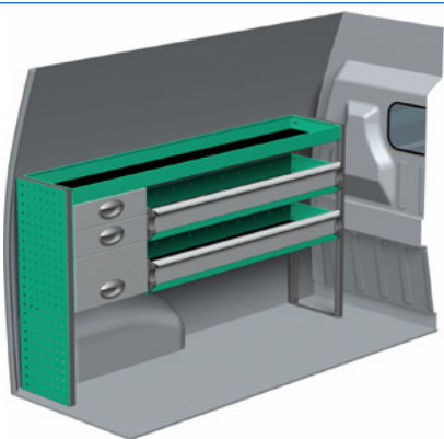
Package number F40082 W x D x H 1633 x 300 x 890 mm • Weight app. 38 kg
