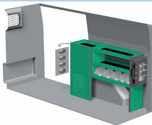
Package number F47043 W x D x H 1372 x 300 x 890 mm • Weight app. 41 kg
