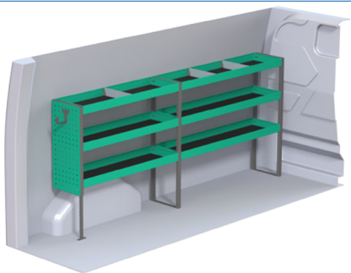
Package number F40720 W x D x H 2270x300x1000 mm • Weight app. 39 kg
