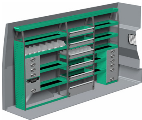
Package number F47084 W x D x H 2873 x 300 x 1735 mm • Weight app. 143 kg
