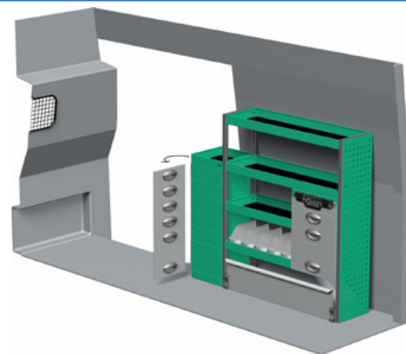
Package number F47063 W x D x H 1362 x 300 x 1220 mm • Weight app. 64 kg
