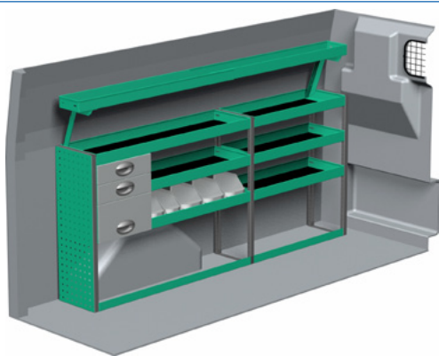
Package number F47044 W x D x H 2057 x 300 x 890/1180 mm • Weight app. 56 kg
