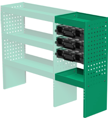
Package number F3279 W x D x H 395 x 300 x 890 mm • Weight app. 9 kg
