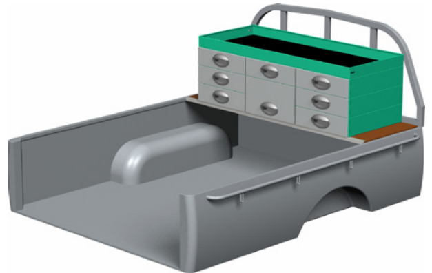
Package number F40105 W x D x H 1176 x 470 x 395 mm • Weight app. 42 kg
