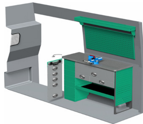
Package number F47065 W x D x H 1330 x 470 x 855 mm • Weight app. 101 kg
