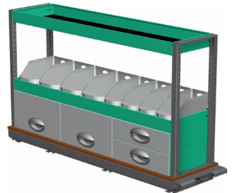
Package number F11033 W x D x H 1300 x 350 x 755 mm • Weight app. 58 kg
