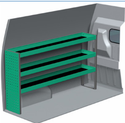
Package number F40080 W x D x H 1633 x 300 x 890 mm • Weight app. 27 kg
