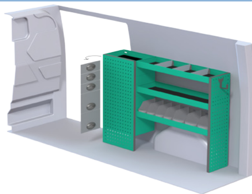
Package number F40721 W x D x H 1500x300x1000 mm • Weight app. 51 kg
