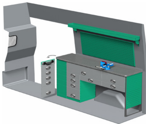
Package number F47085 W x D x H 1935 x 470 x 855 mm • Weight app. 129 kg
