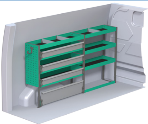
Package number F40702 W x D x H 1878x300x1000 mm • Weight app. 48 kg
