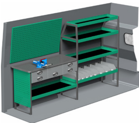
Package number F47066 W x D x H 2449 x 470 x 1510 mm • Weight app. 104 kg
