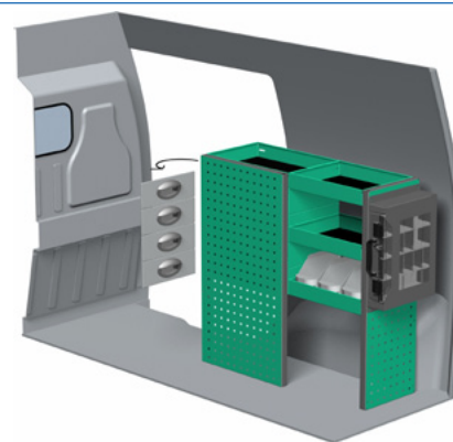
Package number F40083 W x D x H 980 x 300 x 890 mm • Weight app. 36 kg
