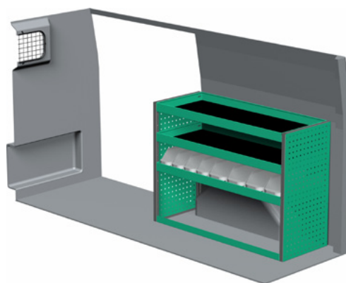
Package number F47047 W x D x H 1242 x 470 x 890 mm • Weight app. 36 kg
