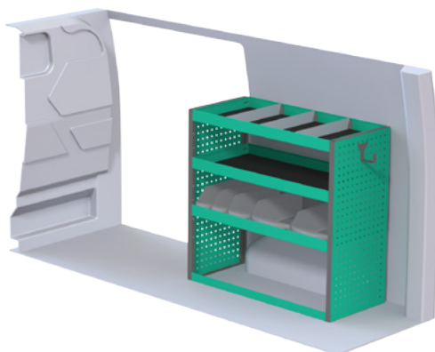
Package number F40707 W x D x H 1063x470x1000 mm • Weight app. 37 kg
