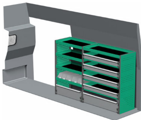
Package number F47087 W x D x H 1879 x 470 x 1220 mm • Weight app. 81 kg
