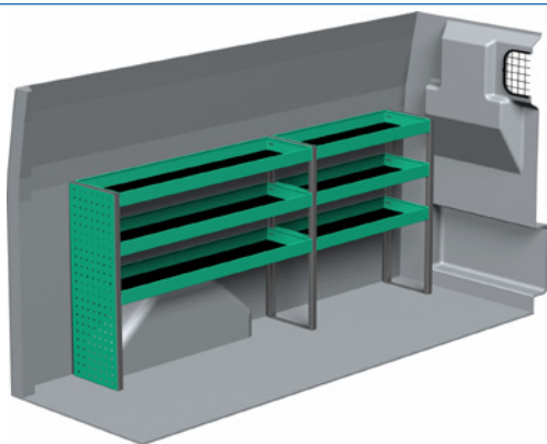
Package number F47040 W x D x H 2057 x 300 x 890 mm • Weight app. 35 kg
