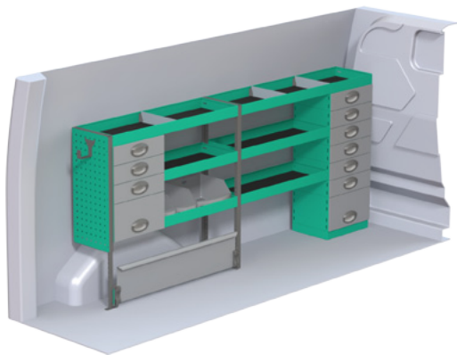
Package number F40726 W x D x H 2238x300x1000 mm • Weight app. 74 kg
