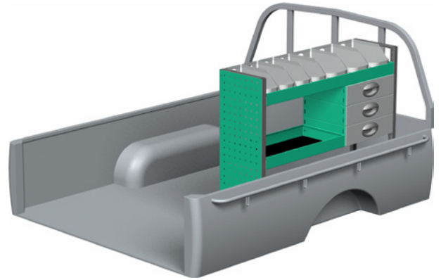
Package number F40101 W x D x H 1062 x 300 x 890 mm • Weight app. 26 kg
