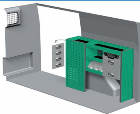
Package number F47045 W x D x H 1287 x 300 x 890 mm • Weight app. 47 kg
