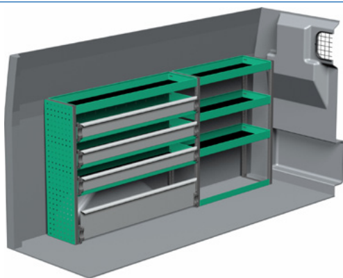
Package number F47042 W x D x H 2057 x 300 x 1000 mm • Weight app. 50 kg
