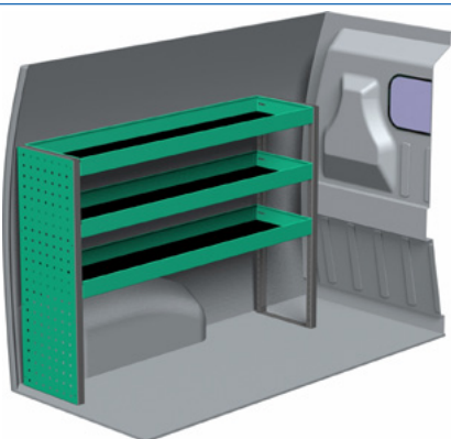
Package number F40060 W x D x H 1241 x 300 x 890 mm • Weight app. 22 kg
