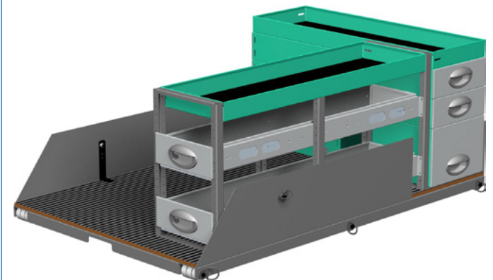
Package number F48081 W x D x H 930 x 1500 x 570 mm • Weight app. 82 kg
