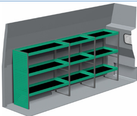
Package number F47080 W x D x H 2873 x 470 x 1220 mm • Weight app. 69 kg
