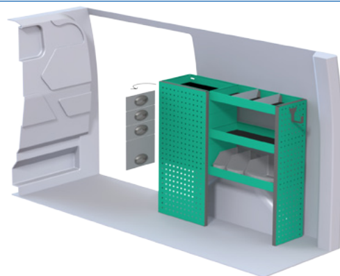
Package number F40701 W x D x H 1108x300x1000 mm • Weight app. 41 kg
