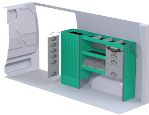
Package number F40725 W x D x H 1500x300x1000 mm • Weight app. 65 kg
