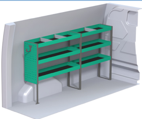
Package number F40700 W x D x H 1878x300x1000 mm • Weight app. 35 kg
