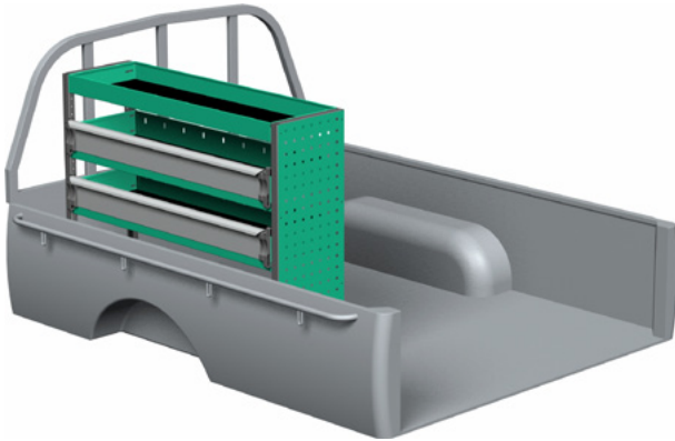
Package number F40102 W x D x H 1062 x 300 x 890 mm • Weight app. 24 kg
