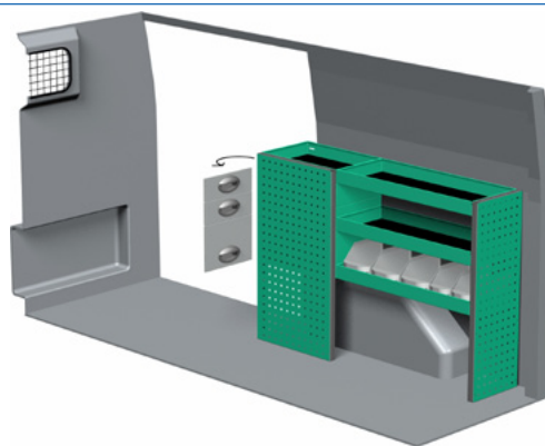
Package number F47041 W x D x H 1287 x 300 x 890 mm • Weight app. 36 kg
