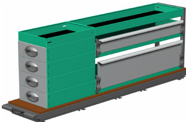
Package number F11035 W x D x H 1650 x 350 x 590 mm • Weight app. 68 kg
