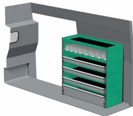
Package number F47067 W x D x H 1242 x 470 x 1220 mm • Weight app. 59 kg
