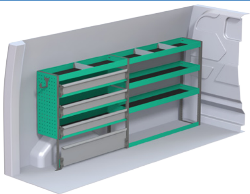
Package number F40722 W x D x H 2270x300x1000 mm • Weight app. 53 kg
