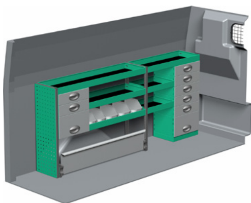
Package number F47046 W x D x H 2025 x 300 x 890 mm • Weight app. 64 kg
