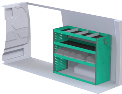
Package number F40727 W x D x H 1242x470x1000 mm • Weight app. 40 kg
