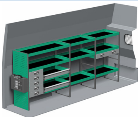
Package number F47082 W x D x H 2958 x 470 x 1220 mm • Weight app. 104 kg
