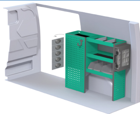
Package number F40703 W x D x H 1197x300x1000 mm • Weight app. 46 kg
