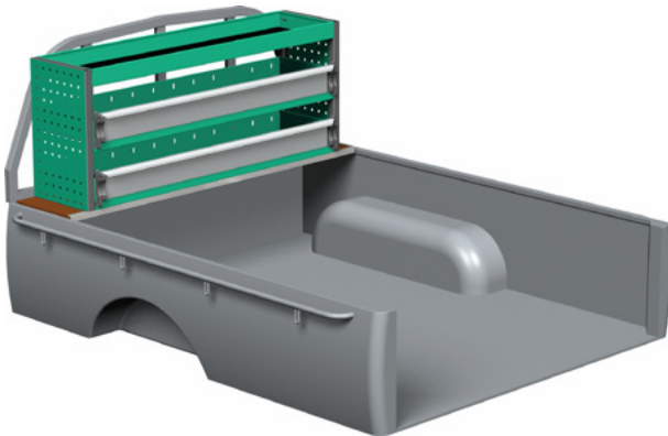
Package number F40104 W x D x H 1242 x 300 x 505 mm • Weight app. 24 kg
