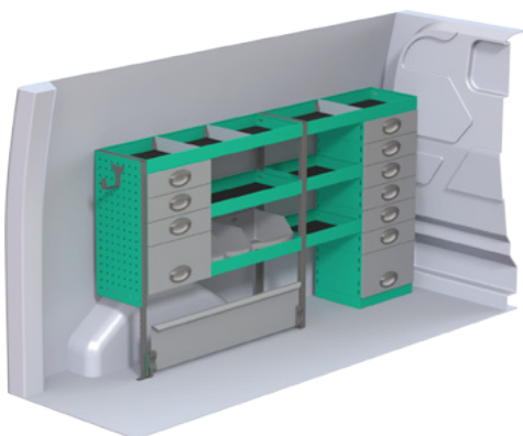
Package number F40706 W x D x H 1846x300x1000 mm • Weight app. 69 kg
